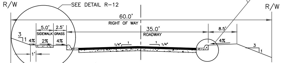
60' RIGHT OF WAY MINOR COLLECTOR 35' ROADWAY SECTION
