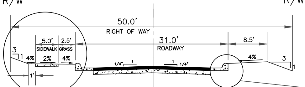
50' RIGHT OF WAY LOCAL STREET 31' ROADWAY SECTION
